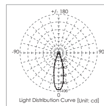
R1001S 1 x 50W IRC 24°
