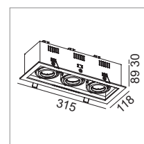
R1003S 3 x 50W IRC 24°
