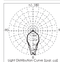
Light Distribution Curve [Unit: cd]
