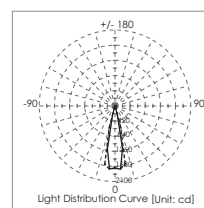
Light Distribution Curve [Unit: cd]
