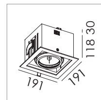
R1020S 1 x 50W IRC 24°
