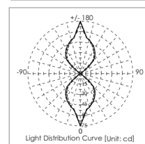
W6019H 2 x 3W
