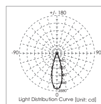
Light Distribution Curve [Unit: cd]
