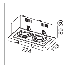
R1002S 2 x 50W IRC 24°
