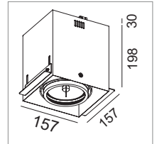
R1019B 1 x 50W IRC 24°
