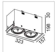
R1029B 2 x 50W IRC 24°
