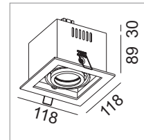
R1001S 1 x 50W IRC 24°
