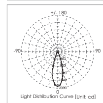
R1039B 3 x 50W IRC 24°
