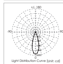
R1003S 3 x 50W IRC 24°
