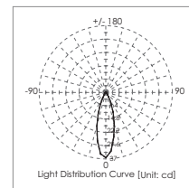
R1018B 3 x 50W IRC 24°
